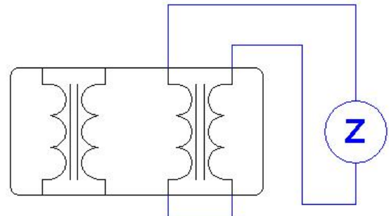
(B):Differential mode
